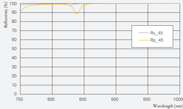
Fig. 3. Polygon Mirror typical data
