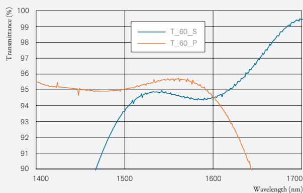
Fig. 5. Cover Window typical data
