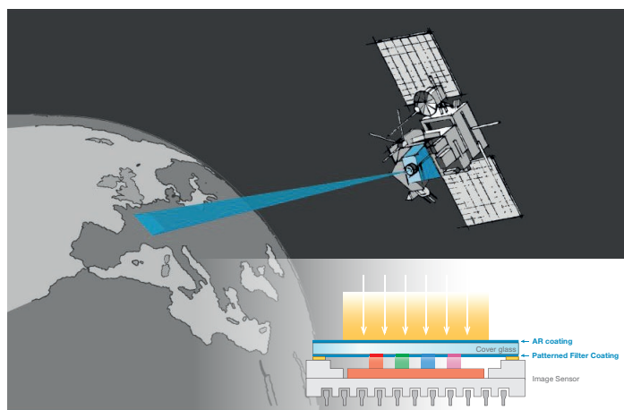
Multi- and Hyperspectral Monitoring from Space
