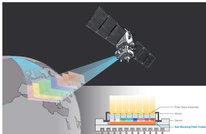
Remote Multi-Spectral Imaging from Space
