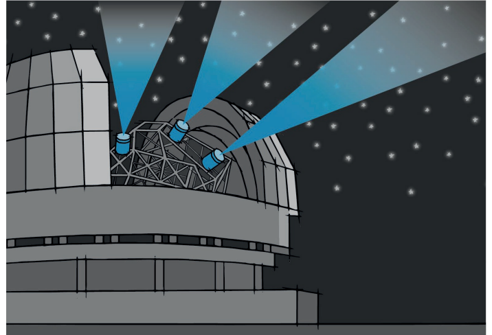
Ground based Astronomical Observation
