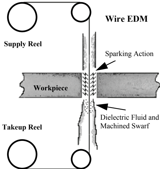
Figure 2 Traveling Wire EDM (TW EDM)
