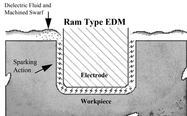
Figure 1 Conventional (RAM) EDM. EDM machines a work piece by forcing a spark through a dielectric fluid from the electrode to the work piece. As each spark impinges on the work piece surface, it removes a minuscule amount of material that is flushed away with the flowing fluid.
